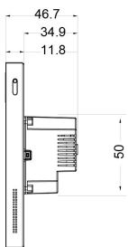
2 RIGHT VIEW
