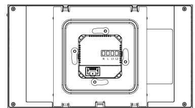
4 BACK VIEW
