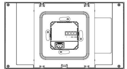
4 BACK VIEW
