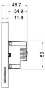
2 RIGHT VIEW
