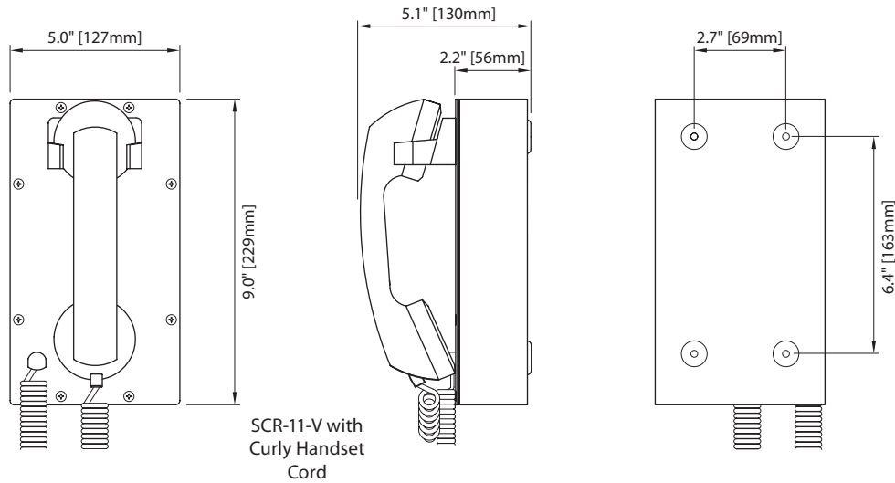
SCR-V Series Steel Compact Ringdown Telephones
